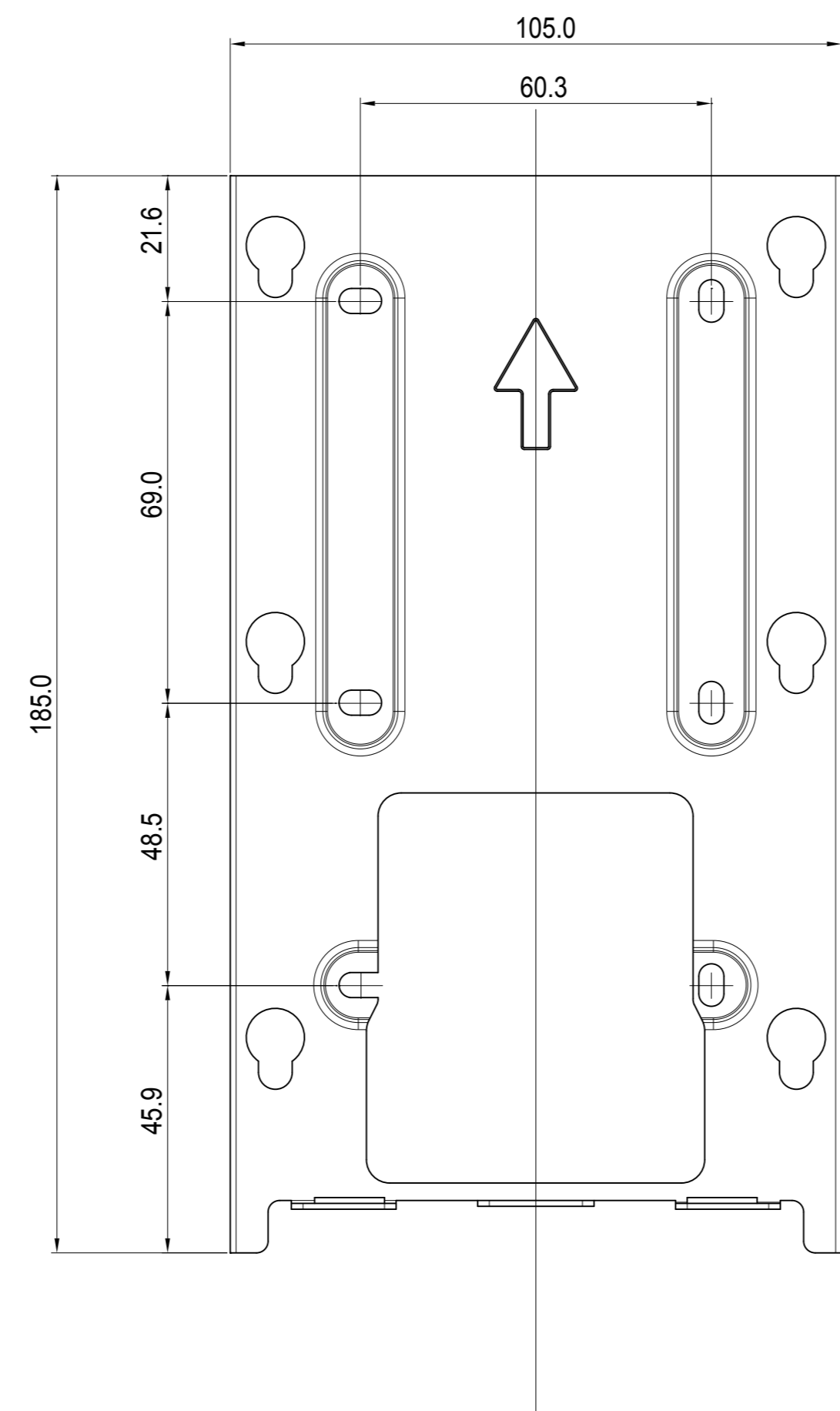
1 FRONT VIEW
