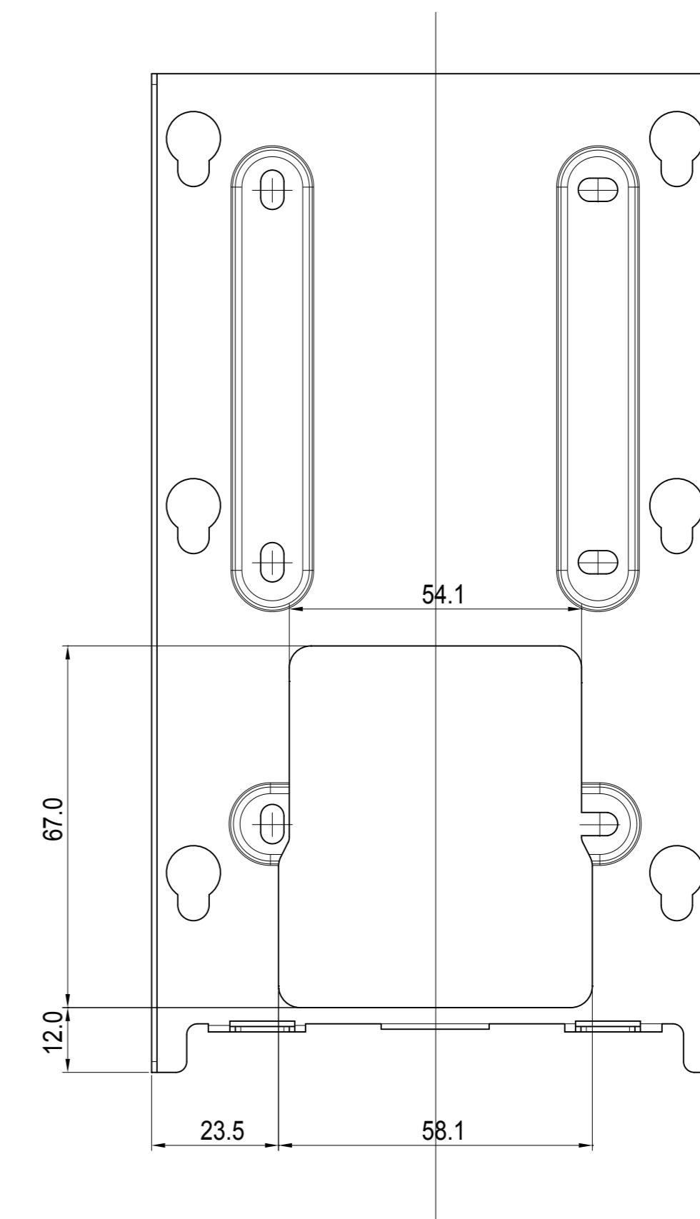
4 BACK VIEW
