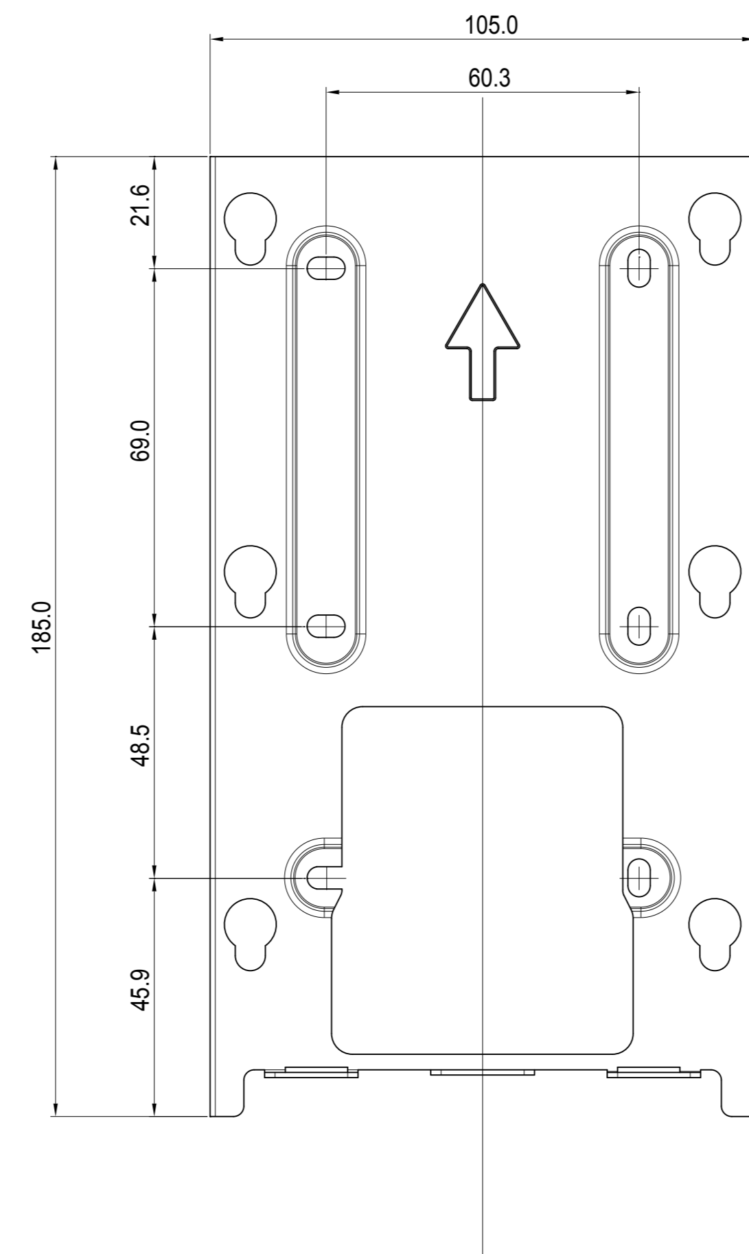
1 FRONT VIEW
